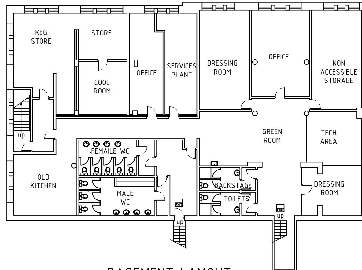
BASEMENT LAYOUT
