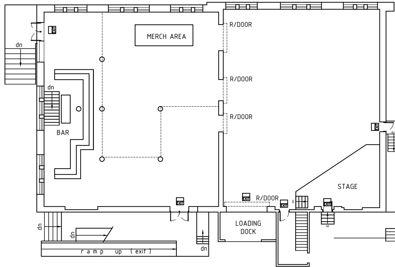
GROUND FLOOR LAYOUT
